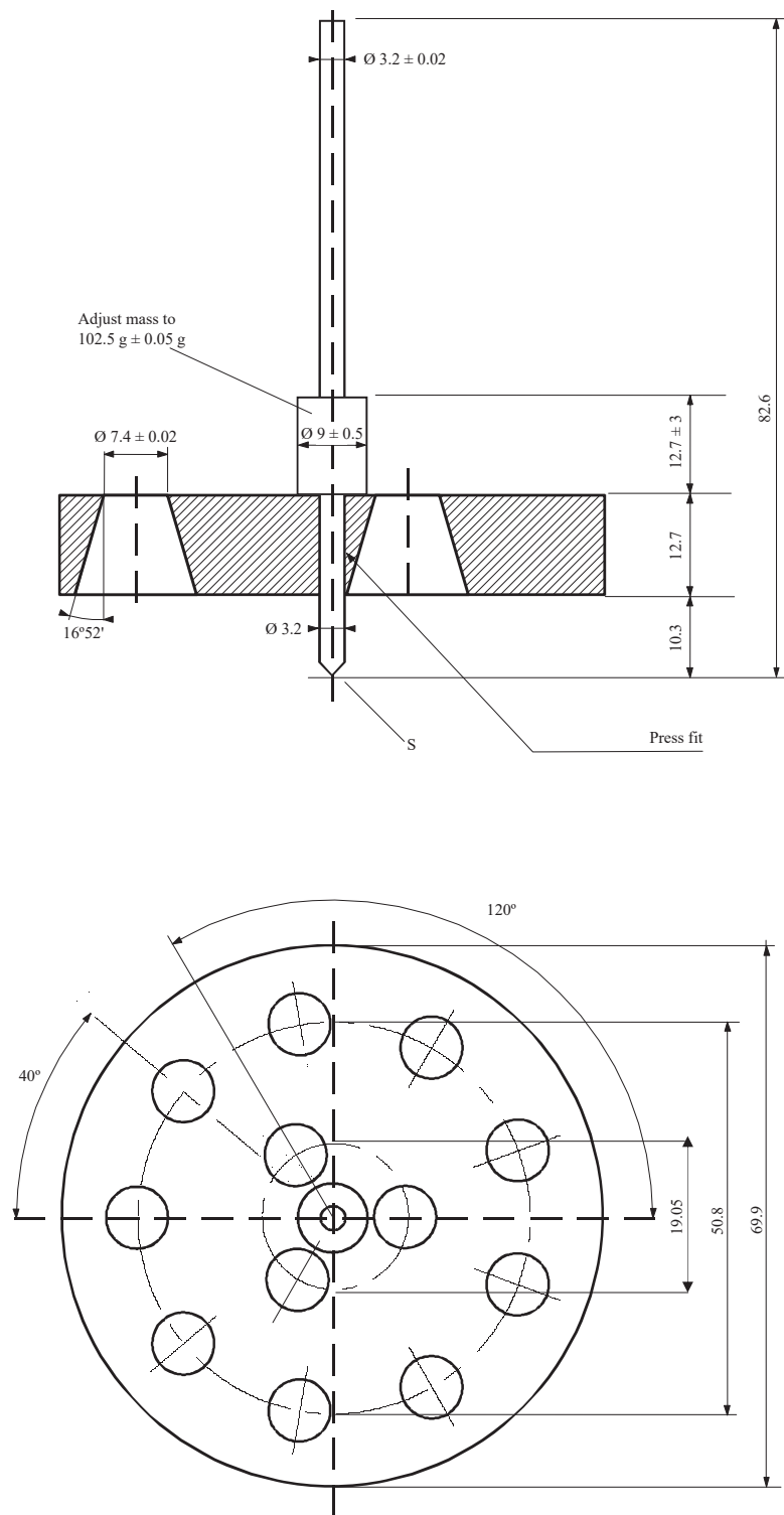
Figure 1 – Penetrometer
